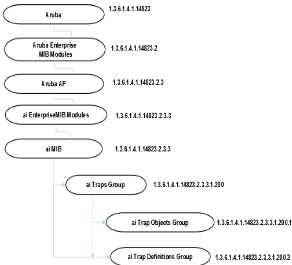
Figure 5 Trap Hierarchy
